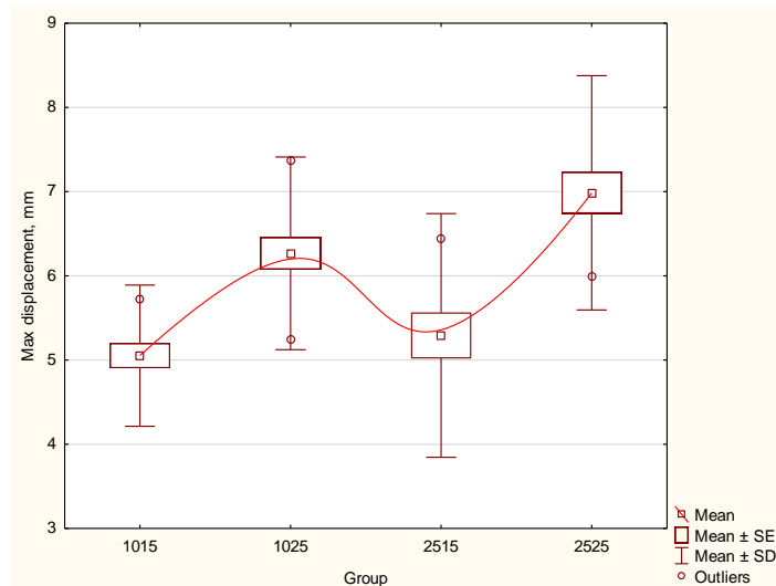
Figure 3. Measurement results of max displacement for 4 specimen groups.
