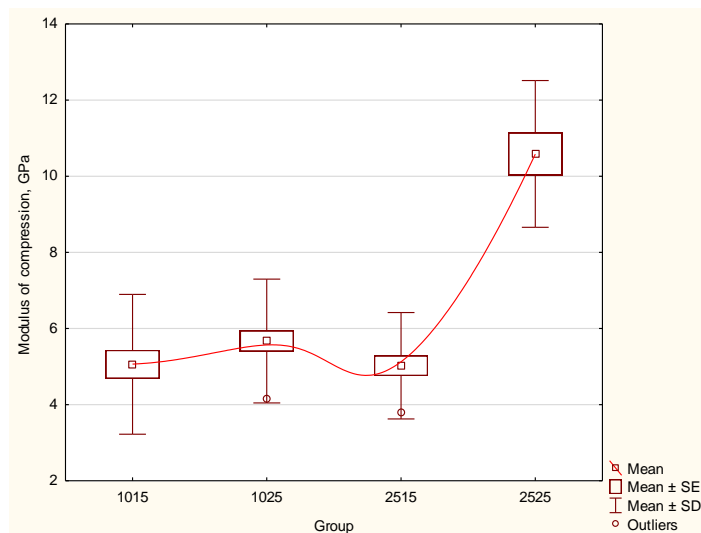
Figure 7. Measurement results of modulus of compression for 4 specimen groups.
