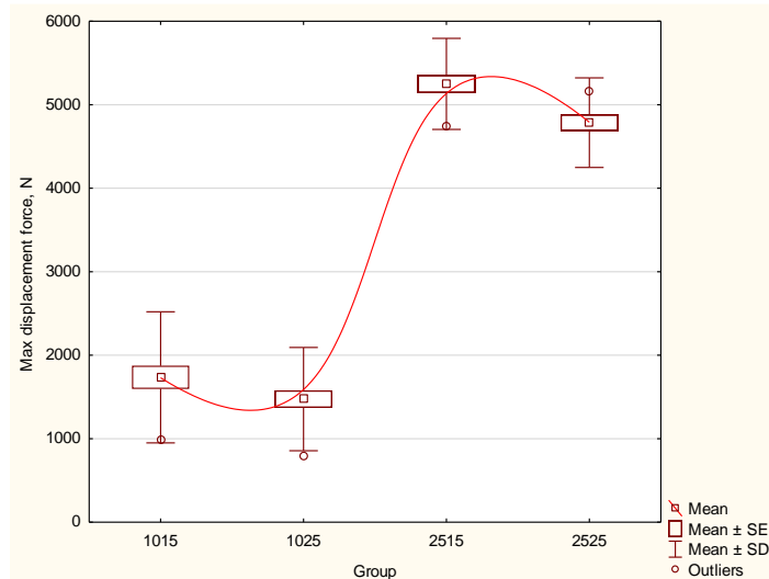
Figure 2. Measurement results of max displacement force for 4 specimen groups.
