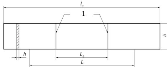
Figure 1. Shape and dimensions of type 2 specimen according to ISO 527-3, here: distance between jaws L : 100 mm \pm 5 mm; width b : from 10 mm to 25 mm; thickness h : \leq 1 mm; total length l_3 : \geq 150 mm.
