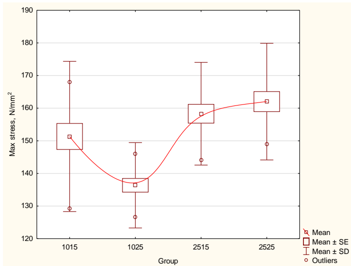
Figure 6. Measurement results of max stress for 4 specimen groups.
