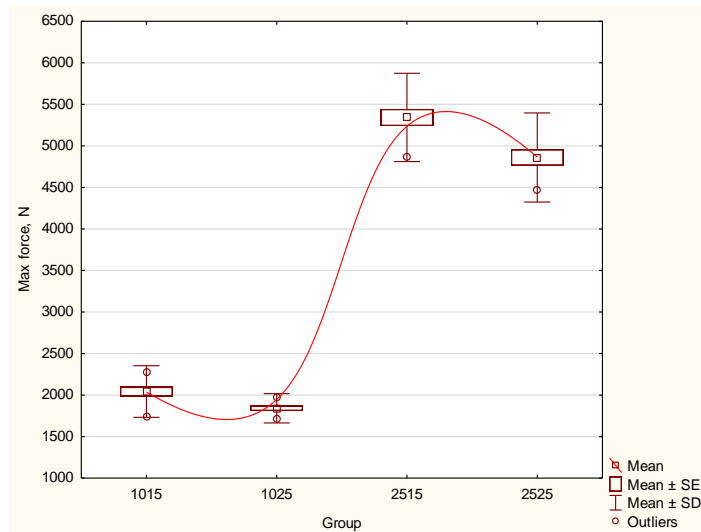
Figure 1. Measurement results of max force for 4 specimen groups.
