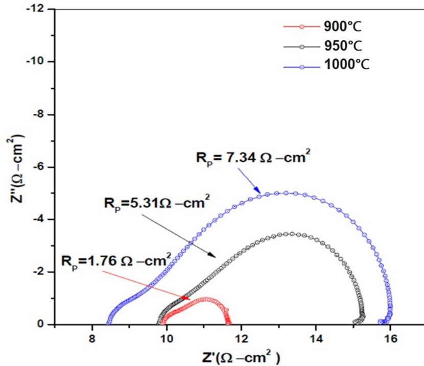
Fig. 3. Impedance spectra of cells with mixed composite cathodes produced at 900, 950 and 1000°C sintering temperatures.
