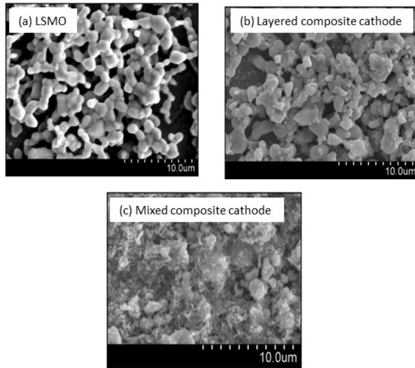
Fig. 1. SEM micrographs of cathode materials: (a) LSMO cathode film sintered at 1330°C, (b) layered composite cathode and (c) mixed composite cathode.
