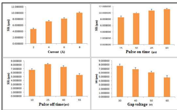
Figure 7. Influence of EDM process factors on SR of composite
