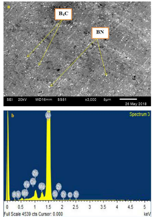
Figure 2. (a-b) SEM micrograph and EDS spectrum of Al7010/2%B 4 C/2%BN HMMNC.
