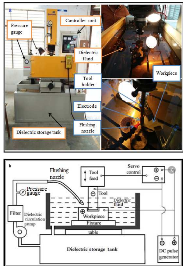
Figure 1. (a) Electrical discharge machine and (b) schematic diagram.
