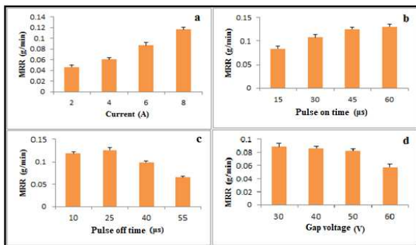
Figure 4. Influence of EDM process factors on MRR for EDM of AA7010/2%B 4 C/2%BN HMMNC.
