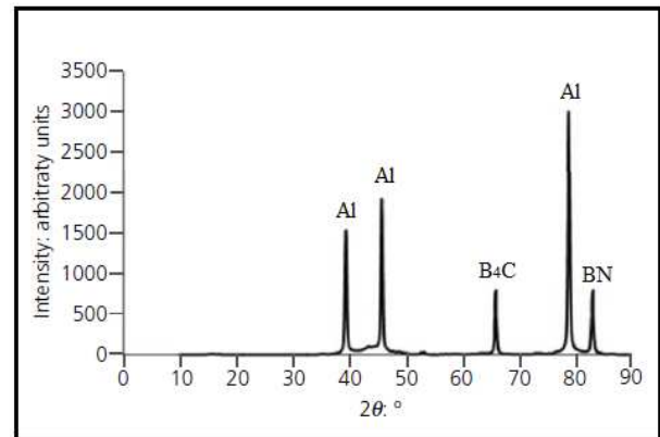
Figure 3. XRD patterns of Al7010/2%B 4 C/2%BN HMMNC.
