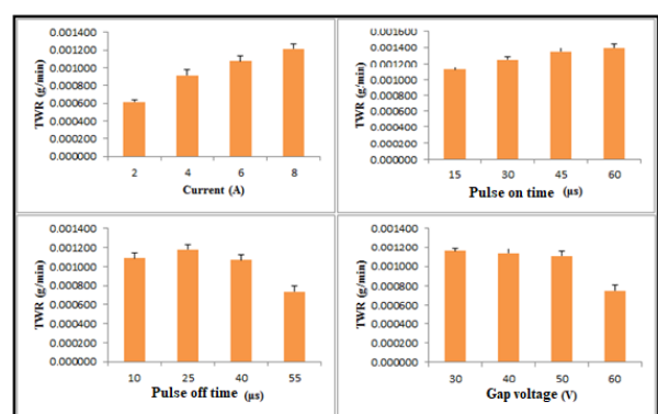
Figure 6. Influence of EDM process factors on TWR for EDM of AA7010/2%B 4 C/2%BN HMMNC.
