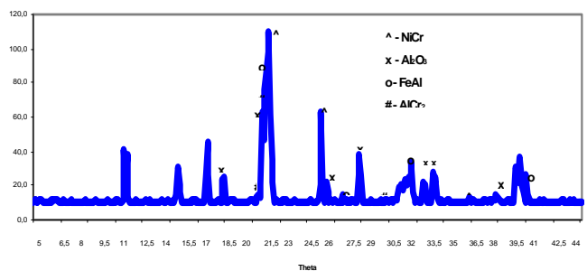
Fig. 4. Diffraction pattern of (NiCr)-FeAl-CrAl-Al 2 O 3 composite powders Rys. 4. Dyfraktogram próbki (NiCr)-FeAl-CrAl-Al 2 O 3
