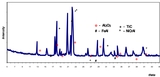
Fig. 2. Diffraction pattern of NiCr-FeAl-TiC-Al 2 O 3 composite powders Rys. 2. Dyfraktogram próbki NiCr-FeAl-TiC-Al 2 O 3
