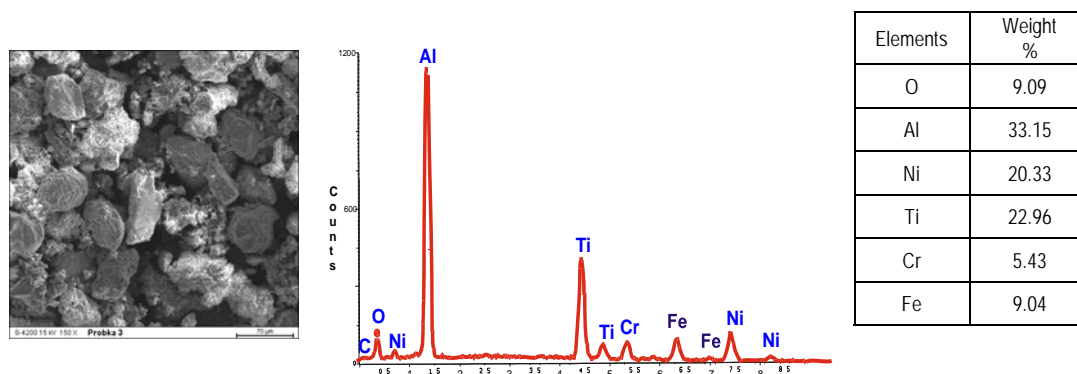
Fig. 7. Morphology (SEM) and a spectrum of characteristic X-ray from NiCr-FeAl-TiAl-Al 2 O 3
