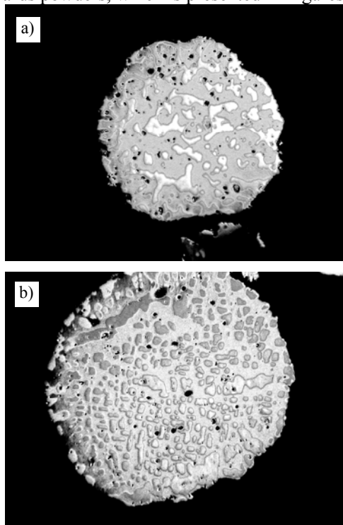
Fig. 1. Structure of composite powders: a) (NiCr)-FeAl-CrAl-Al 2 O 3 , b) (NiCr)-FeAl-Cr 3 C 2 -Al 2 O 3
