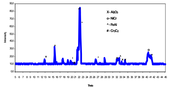
Fig. 5. Diffraction pattern of NiCr-FeAl-Cr 3 C 2 -Al 2 O 3 composite powders Rys. 5. Dyfraktogram próbki NiCr-FeAl-Cr 3 C 2 -Al 2 O 3
