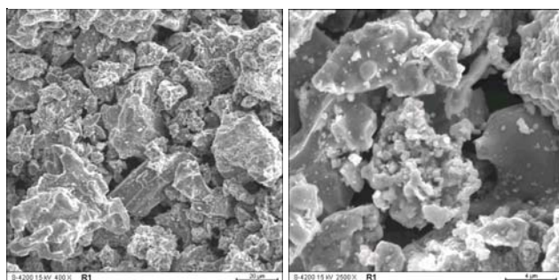
Fig. 8. Composite powder morphology of NiCr-FeAl-CrAl-Al 2 O 3
