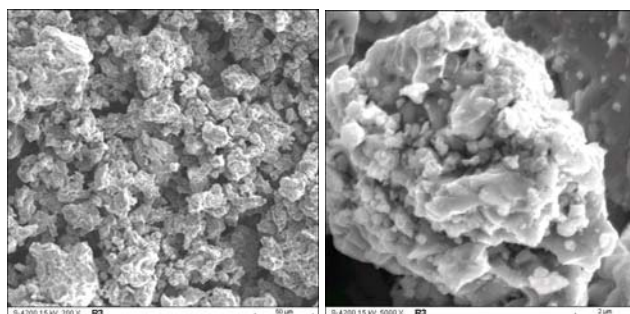
Fig. 9. Composite powder morphology NiCr-FeAl-Cr 3 C 2 -Al 2 O 3
