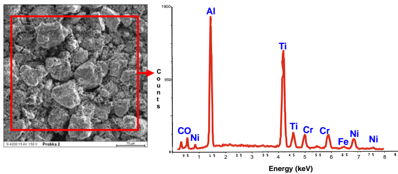
Fig. 6. Morphology (SEM) and a spectrum of characteristic X-radiation (EDX) from NiCr-FeAl-TiC-Al 2 O 3 Rys. 6. Morfologia (SEM) i EDX próbki NiCr-FeAl-TiC-Al 2 O 3
