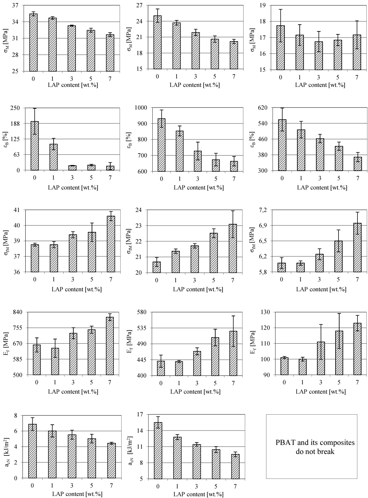
Fig. 2. Mechanical properties of studied samples (PBS-based samples – left column, PCL-based samples – middle column and PBAT-based samples – right column)
