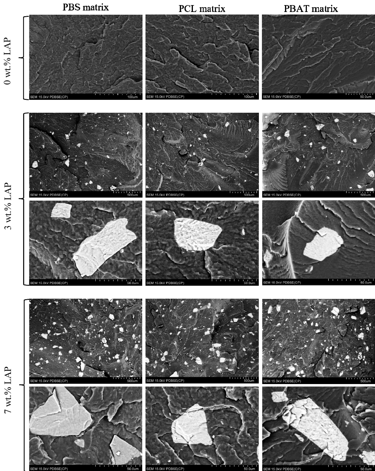
Fig. 1. SEM micrographs of PBS (left column), PCL (middle column) and PBAT (right column) composites; lower and higher magnification images are shown for composites with 3 wt.% and 7 wt.% LAP
